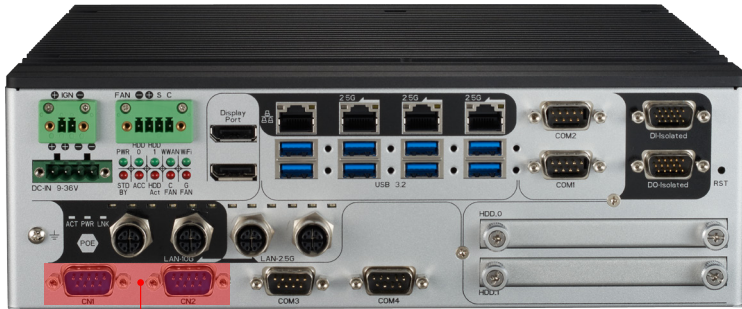
CAN BUS Ports
